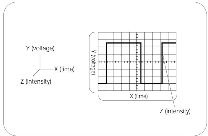
▶ Figure 2. X, Y, and Z components of a displayed waveform.
